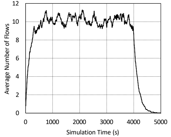
Fig. 3. Example of the average number of flows passing a link versus simulation time for Traffic #1.
