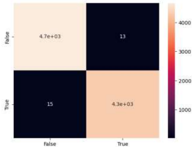
Accuracy score graph for decision tree
