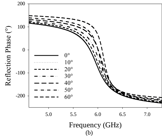
Fig. 4. (a) Magnitude and (b) phase of Square-Ring Octagonal AMC with DGS when applied to different incidence angle from 0^\circ to 60^\circ .
