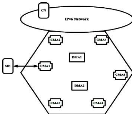
Fig. 1. Architecture of SIDP.
