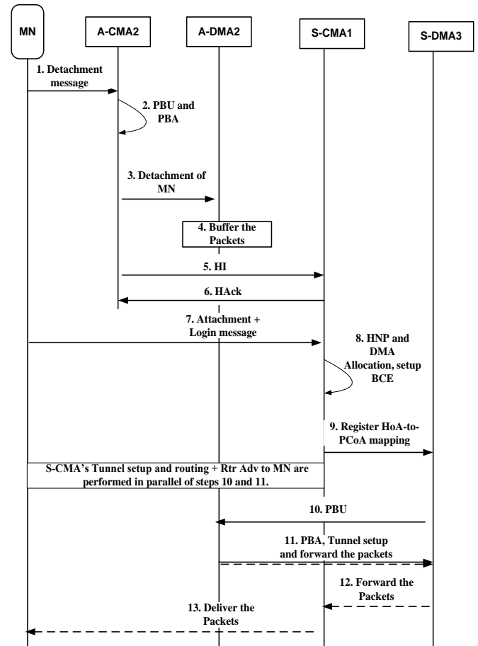
Fig. 6. Signaling flow for the SIDP handover process.
