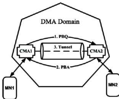
Fig. 3. Routing optimization scheme.
