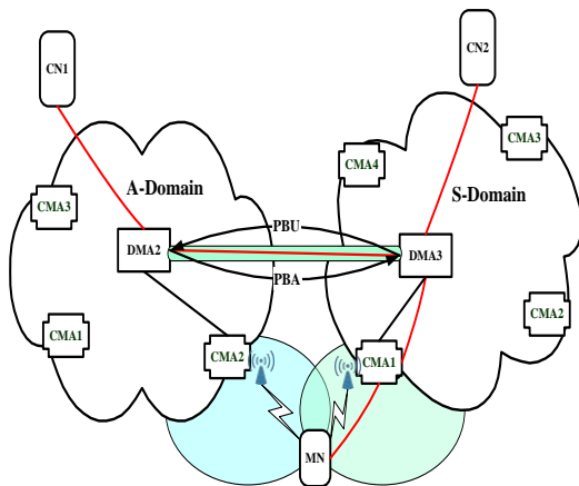
Fig. 5. Inter-domain handover process for SIDP.
