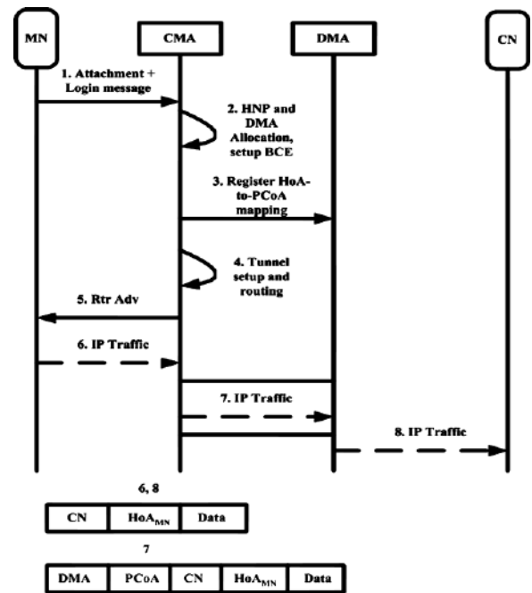
Fig. 2. Basic design for deployment of SIDP.
