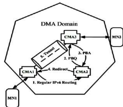
Fig. 4. Assumption of CMA2 as an anchor for optimized routing.
