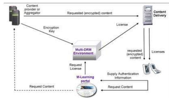
Fig. 1. Basic mobile learning use case with the DRM architecture
