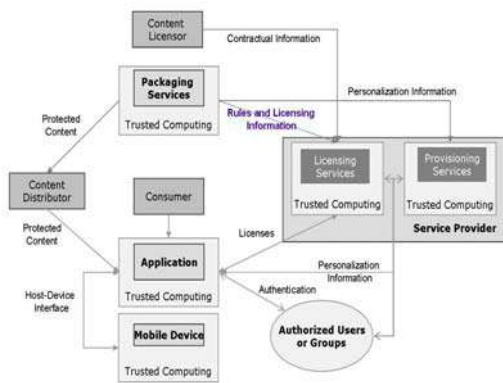
Fig. 2. DRM elements architecture
