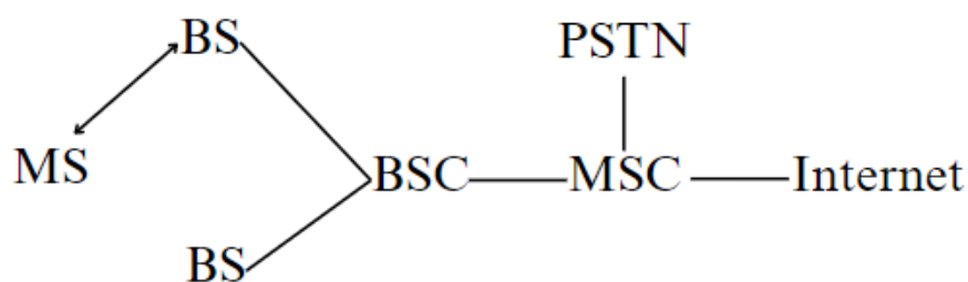
Figure 1. The architecture of AMPS
