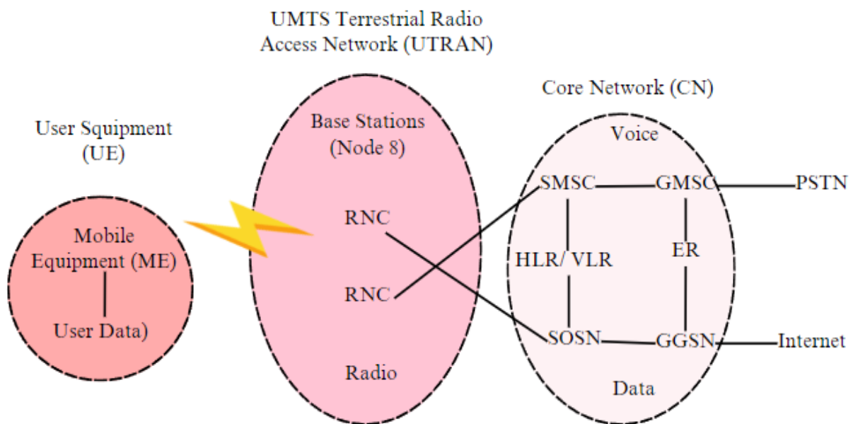
Figure 4. Diagram of the WCDMA Network
