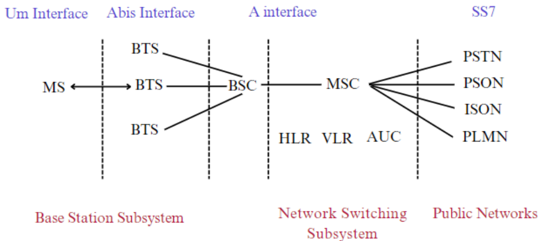
Figure 2. Architecture of the GSM System
