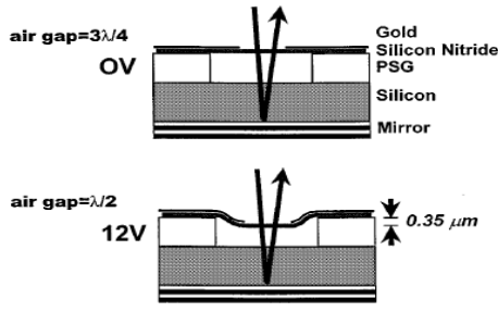
Fig. 5. MEMS all-pass filter schematic showing the change in air gap with applied voltage [14].
