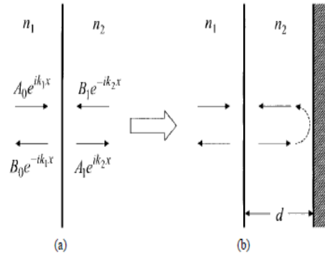
Fig .4. Thin-film example: (a) Interface between two dielectrics. The scattering matrix relates the “input” amplitudes A_0 and B_1 to the “output” amplitudes A_1 and B_0 . (b) By connecting the “output” A_1 to the “input” B_1 through a delay (using a 100% reflector a distance d away), a single-stage APF is obtained. This is exactly the familiar Gires–Tournois interferometer [12].
