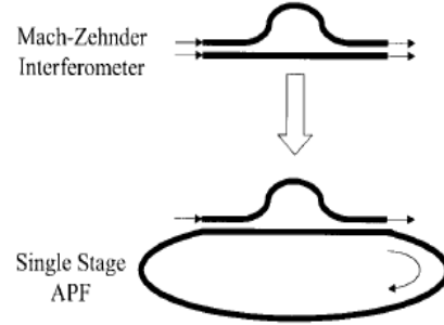
Fig 3. Single stage APF using Mach-Zehnder interferometer [12]
