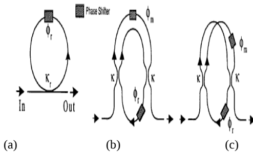
Fig. 6. (a) Ring resonator all-pass filter with a fixed coupling ratio, and fully tunable ring resonator all-pass filters with (b) an asymmetric MZI and (c) a symmetric MZI [15].
