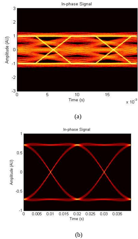
Fig. 7 (a) Eye diagram of the dispersion affected signal (b) Eye diagram of same diagram compensated with RCF
