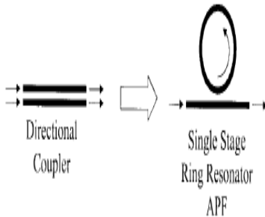
Fig 1. Single stage APF using directional coupler [12].
