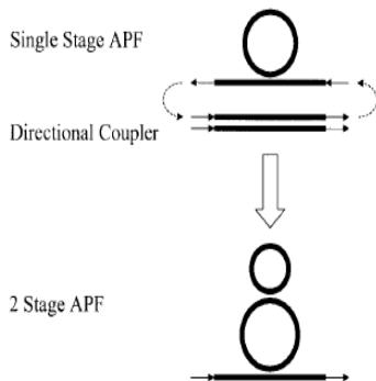
Fig 2. Two stage APF [12].
