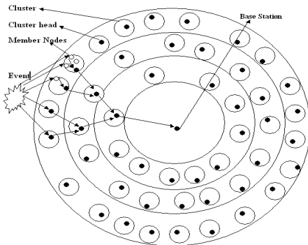
Fig. 3. Shows the message flow from the event point to the base station. The dark circle in the cluster represents the cluster head and hollow circles represent member nodes.
