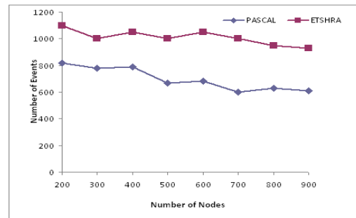
Fig. 7. ETSHRA vs. PASCAL
