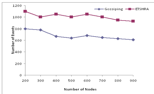
Fig. 6. ETSHRA vs. gossiping.
